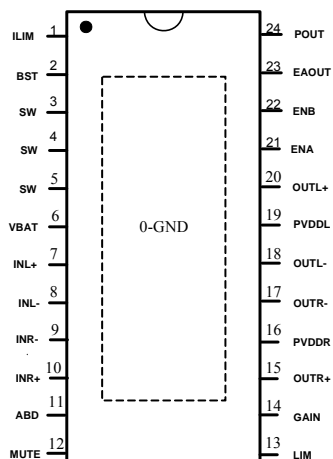
HT878 Top View
