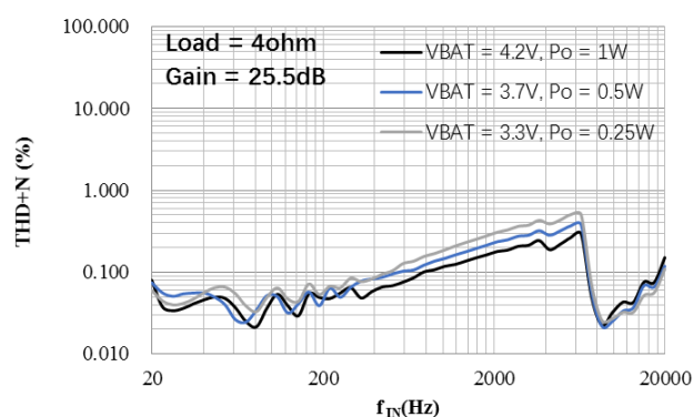
f_{IN} vs THD+N
