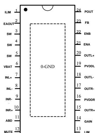
HT878T Top View
