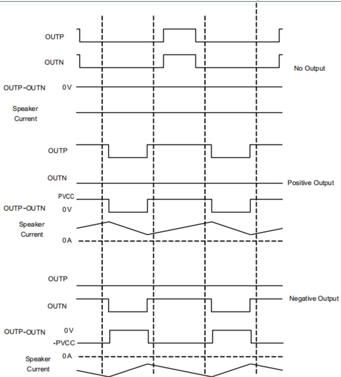
Figure 8 1SPW Modulation
