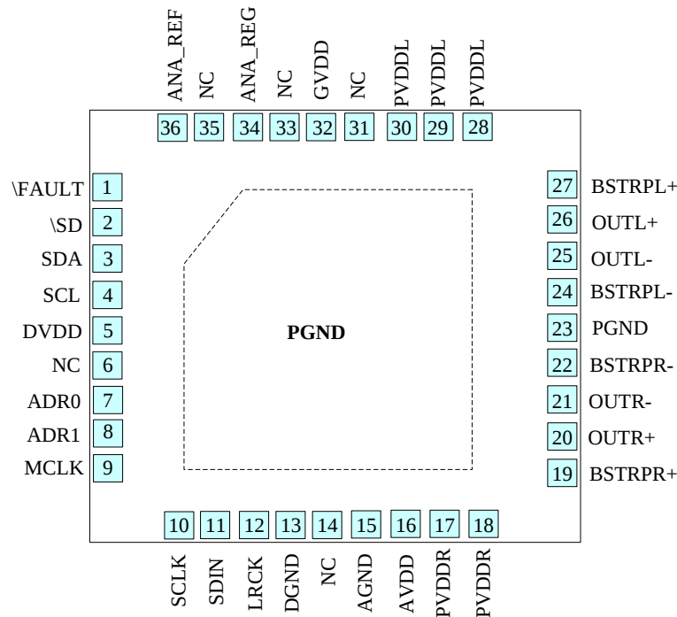
Top View
