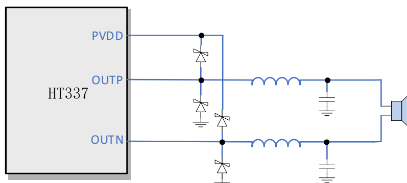
Figure 5 Place Schottky Diodes in the Output Terminals
