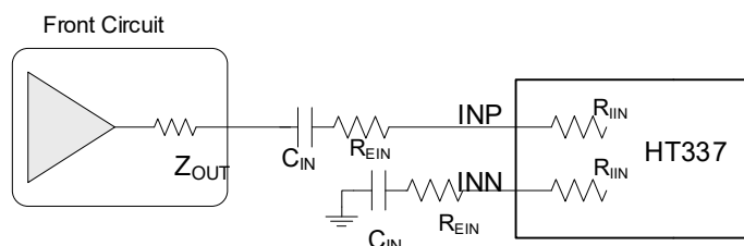
Figure 2 Single-ended Input configuration
