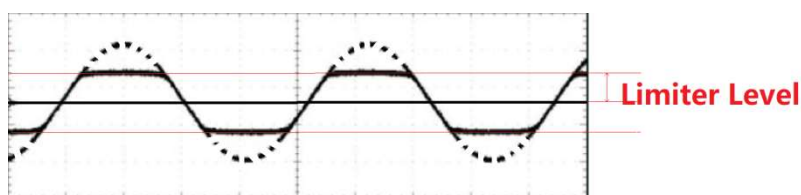
Figure 7 PLIMIT Function Description
